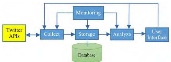
Fig. 1. A generic architecture for Twitter Data Analytics
